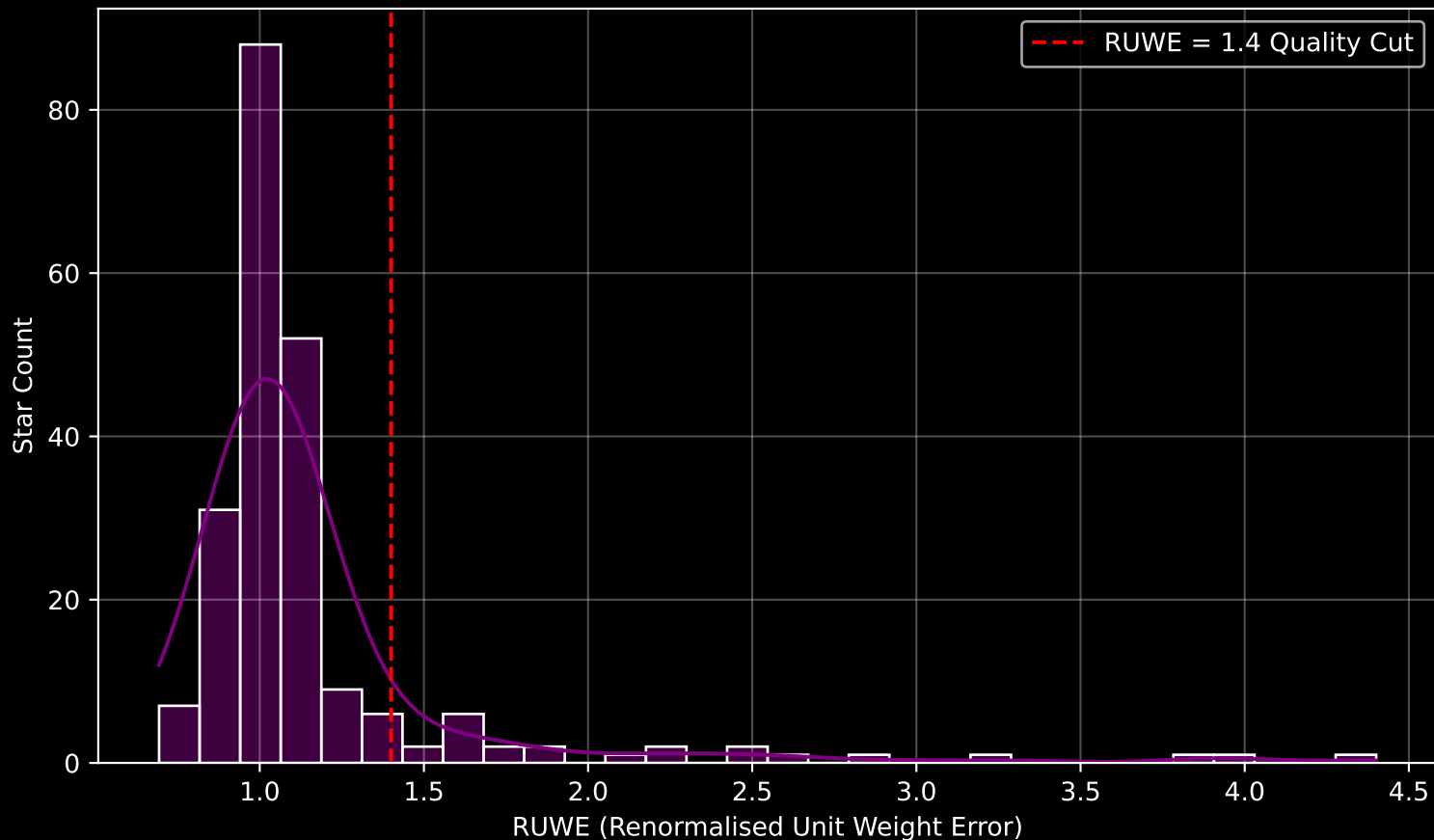
GAPOGEE DR17 Field [067-47_MGA] RUWE Distribution (n= 216)
