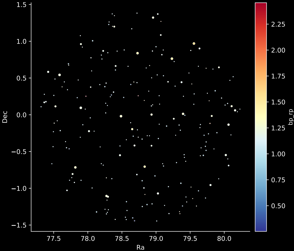
APOGEE DR17 Field: [067-47_MGA] Stars: 224
