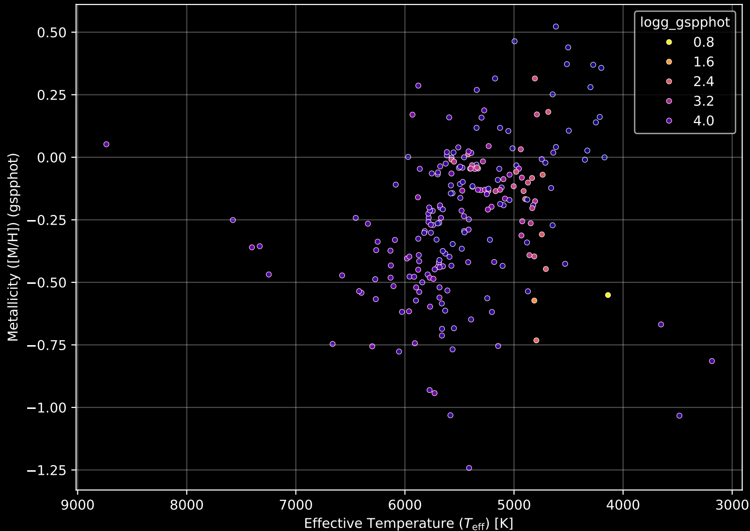
APOGEE DR17 Field: [067-47_MGA] Stellar Population Parameters (n= 224)
