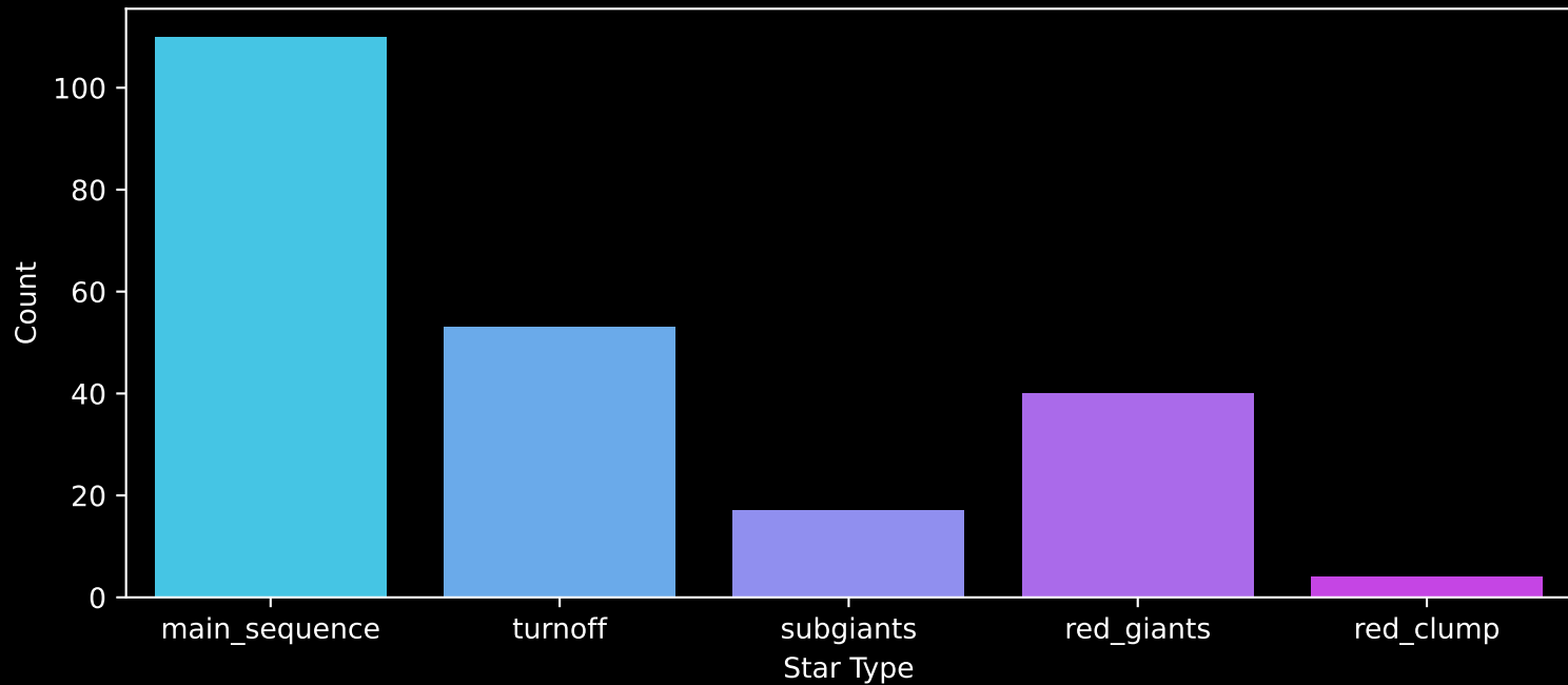
APOGEE DR17 Field: [067-47_MGA] Count plot of Star Type
