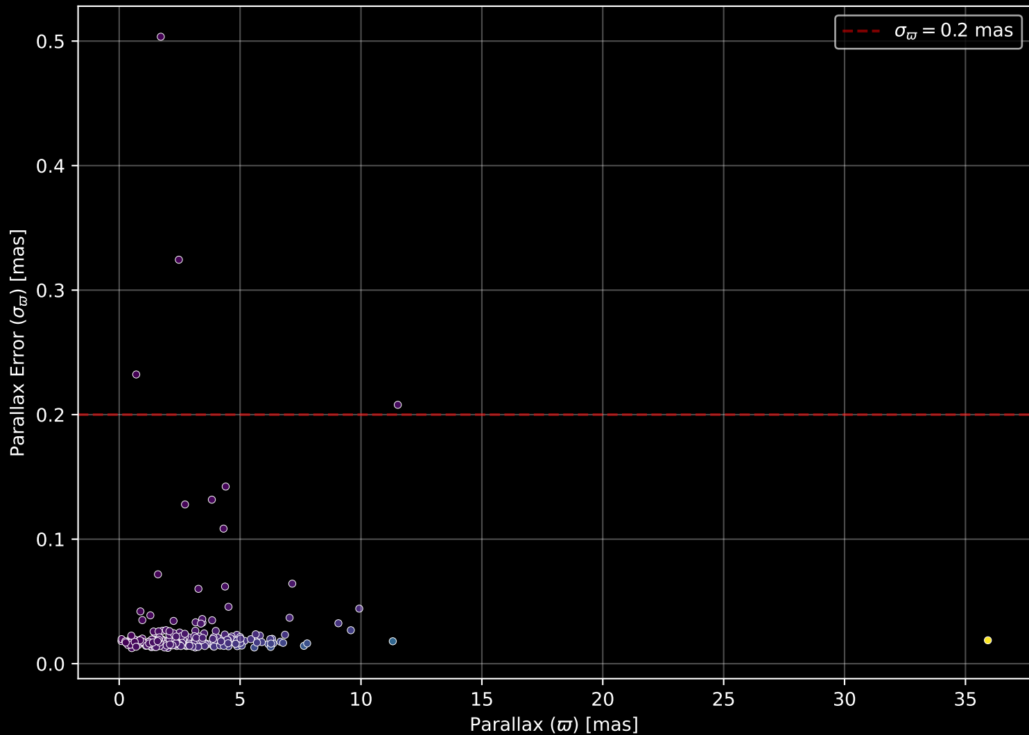
APOGEE DR17 Field: [067-47_MGA] Parallax Quality (n= 224)
