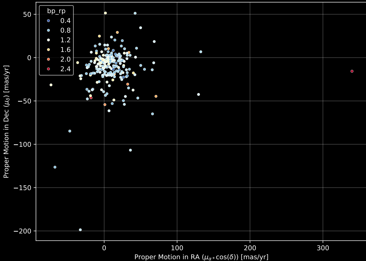
APOGEE DR17 Field: [067-47_MGA] Proper Motion Diagram (n= 224)
