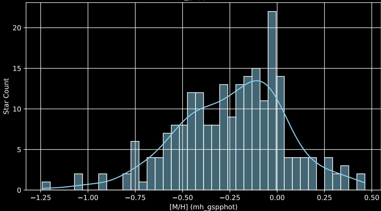
APOGEE DR17 Field: [067-47_MGA [M/H] (mh_gspphot) (n= 223)
